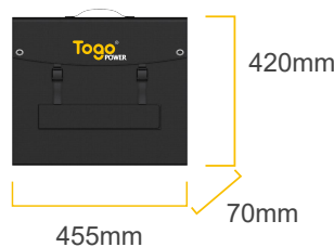
Solar Charger (Folded Dimension)
