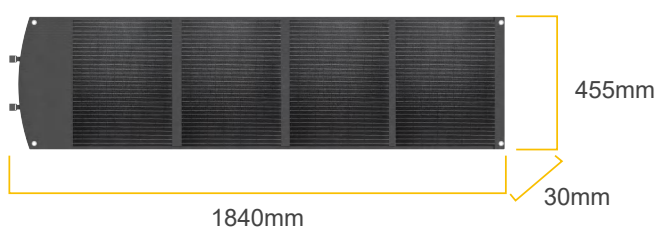
Solar Charger (Unfolded Dimension)
