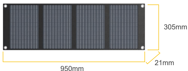
Solar Charger (Unfolded Dimension)
