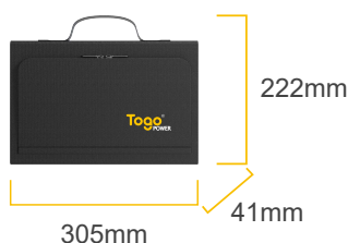
Solar Charger (Folded Dimension)
