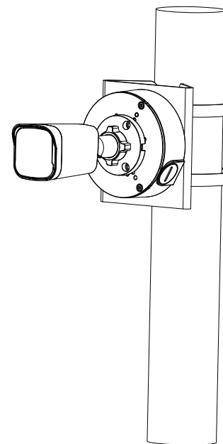
Pole Mount(Vertical)
