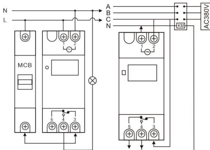
Single phase 220V
