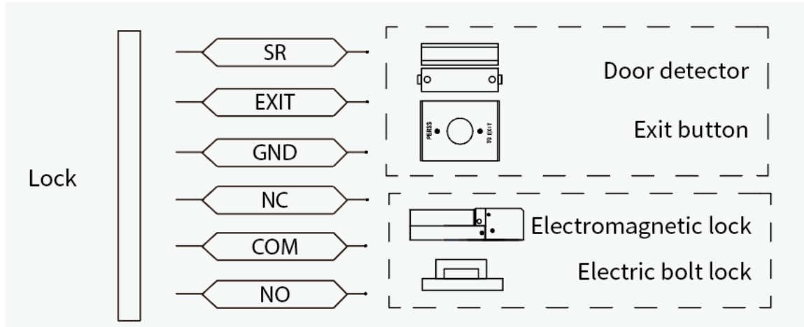
Figure 3-1 Wiring
