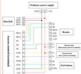
【2】 If it's general power supply, the lock could connect the access controller directly.
