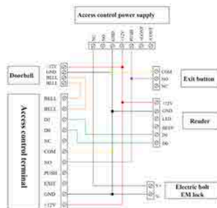
【1】 Connecting professional access control power supply (the lock connect with power supply)
