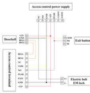
【1】 Connecting professional access control power supply (the lock connect with power supply)
