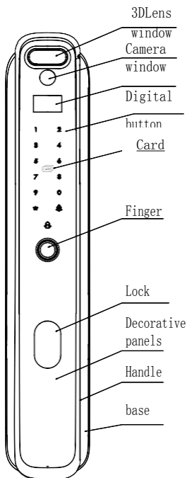
Front panel
