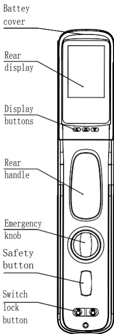
Back panel
