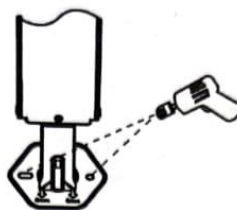
2. According to the size of the base mounting hole, make two mounting holes on the wall.
