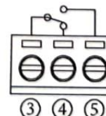
COM NC NO ALARM
